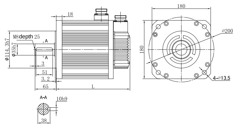
SV-SM18-7R5B shaft extension dimension (unit: mm)
